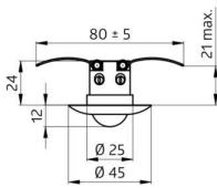
sensor head
