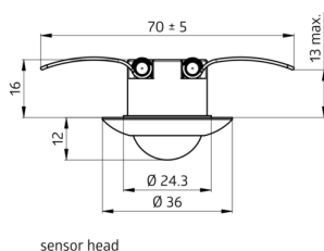
sensor head
