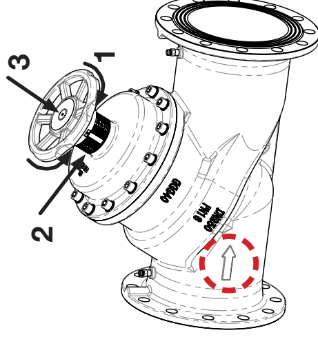
DN200-DN250-DN300
