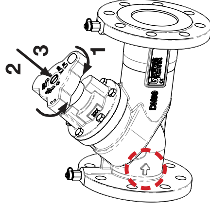
DN65-DN80-DN100-DN125-DN150
