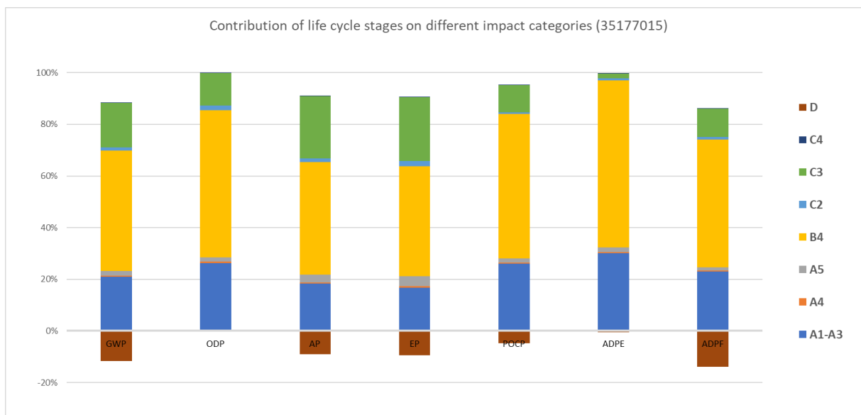
Figure 2: Contribution of the different life cycle stages to the environmental impact of one m 2 of Alkorplan L (35177015).
