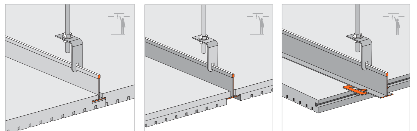
PERFIL OCULTO T-15 T-15 (9/16") concealed grid PERFIL SEMIVISTO T-15/T-24 T-15 (9/16") or T-24 (15/16") semi-exposed grid PERFIL OCULTO T-24 + GRAPA T-24 (15/16") concealed grid + cramp
