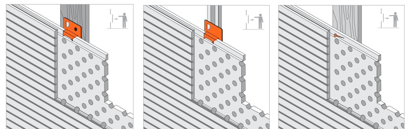
RASTREL MADERA + GRAPA WOODEN STRIP + CRAMP PERFIL OMEGA + GRAPA OMEGA PROFILE + CRAMP RASTREL MADERA WOODEN STRIP
