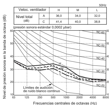
MML-UP0151BH-E, MML-UP0181BH-E
