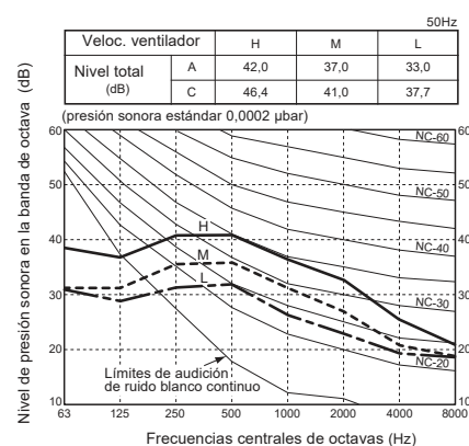
MML-UP0241BH-E
